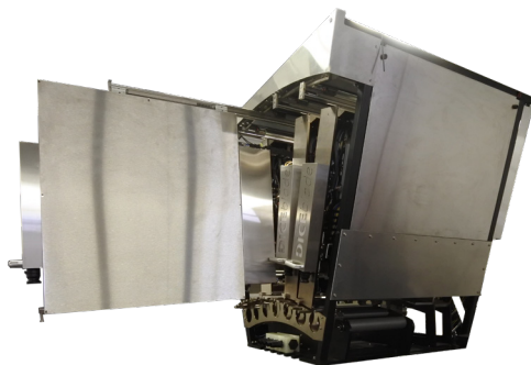
DICEweb with blade in maintenance position
